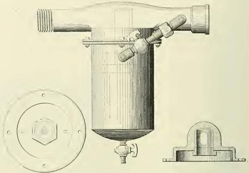
MORRISON AUTOMATIC SAFETY VALVE.
